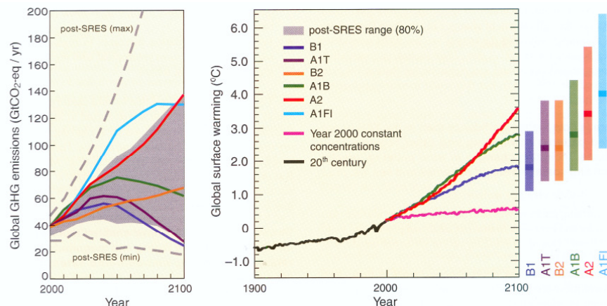
Figure 2 (Figure SPM.5 from the IPCC AR4 Synthesis Report). Left Panel: Global GHG emissions (in GtCO 2 -eq) in the absence of climate policies: six illustrative SRES 7 marker scenarios (coloured lines) and the 80th percentile range of recent scenarios published since SRES (post-SRES) (gray shaded area). Dashed lines show the full range of post-SRES scenarios. The emissions include CO 2 , CH 4 , N 2 O and F-gases. Right Panel: Solid lines are multi-model global averages of surface warming for scenarios A2, A1B and B1, shown as continuations of the 20 th - century simulations. These projections also take into account emissions of short-lived GHGs and aerosols. The pink line is not a scenario, but is for Atmosphere-Ocean General Circulation Model (AOGCM) simulations where atmospheric concentrations are held constant at year 2000 values. The bars at the right of the figure indicate the best estimate (solid line within each bar) and the likely range assessed for the six SRES marker scenarios at 2090-2099. All temperatures are relative to the period 1980-1999. To express the change relative to the period 1850-1899 add 0.5°C.
